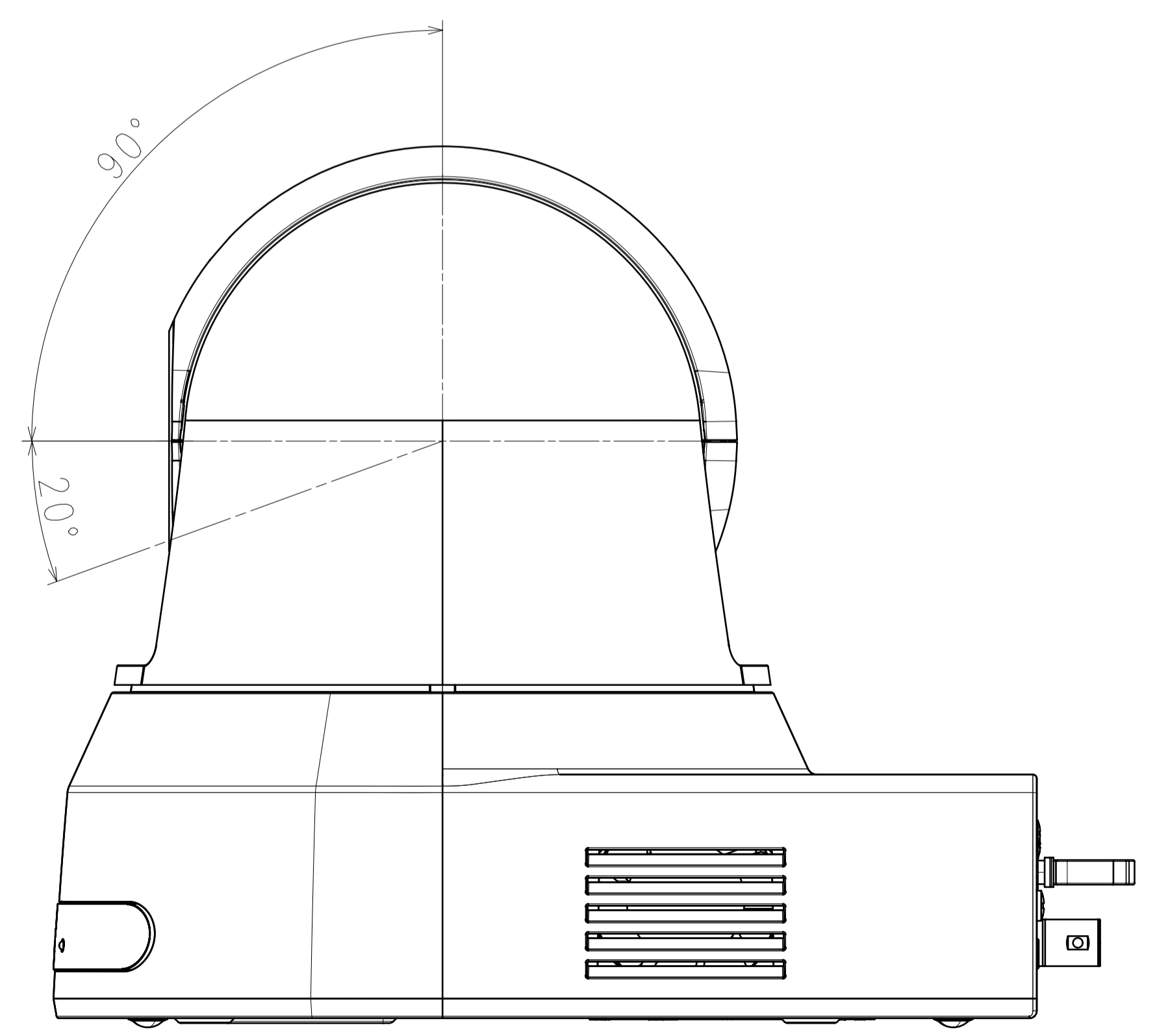
SIDE VIEW
