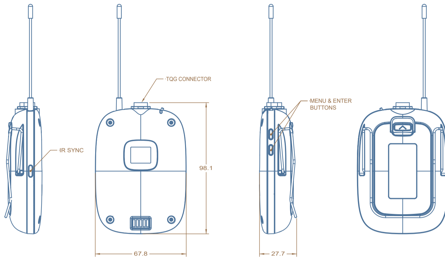
SHURE SLXD1 SCALE 1:1 DIMENSIONS IN mm
