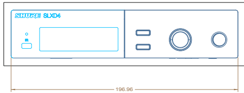
SHURE SLXD4 SCALE 1:1 DIMENSIONS IN mm
