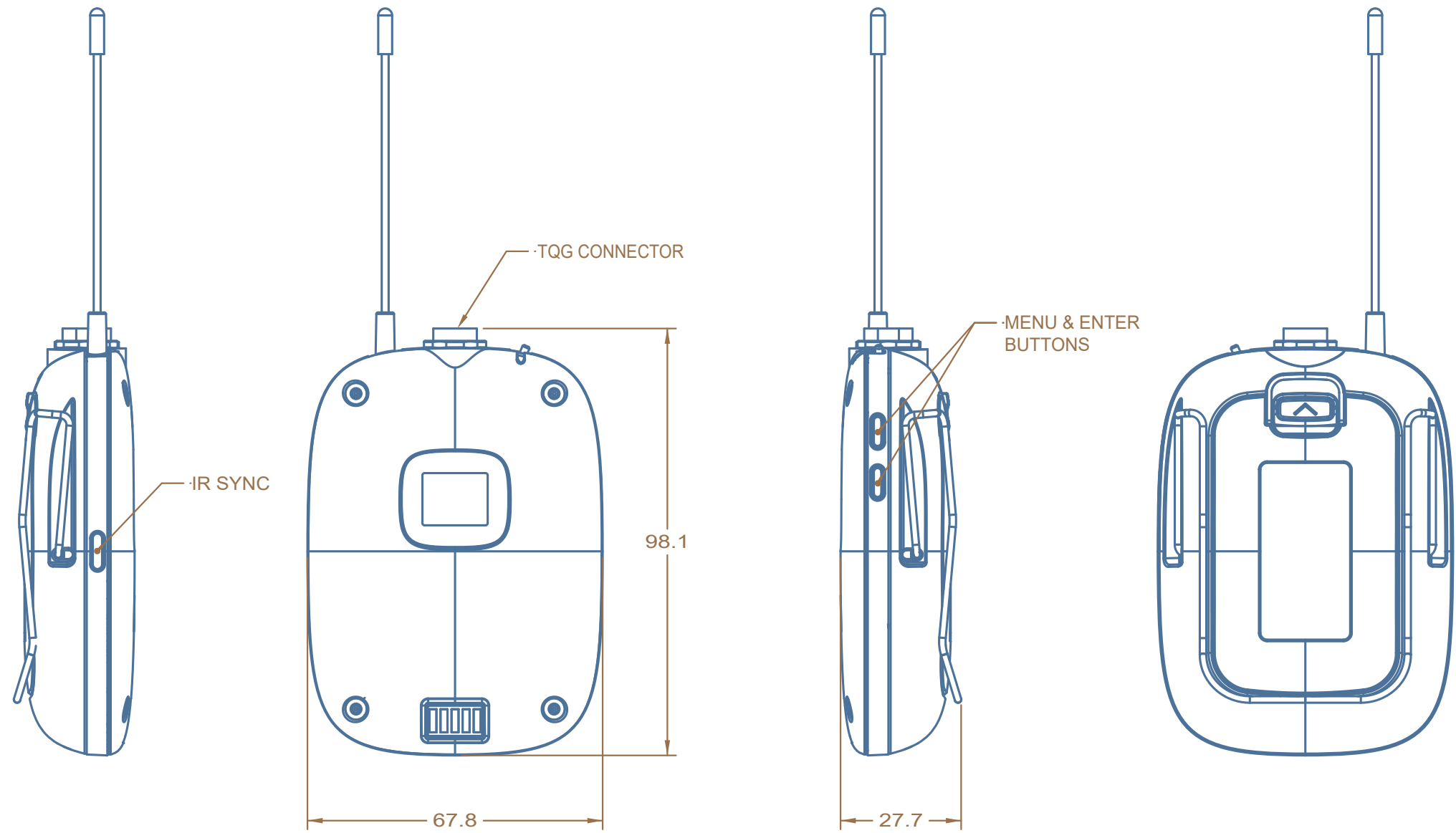
SHURE SLXD1 SCALE 1:1 DIMENSIONS IN mm
