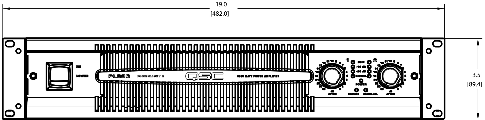
FRONT VIEW
