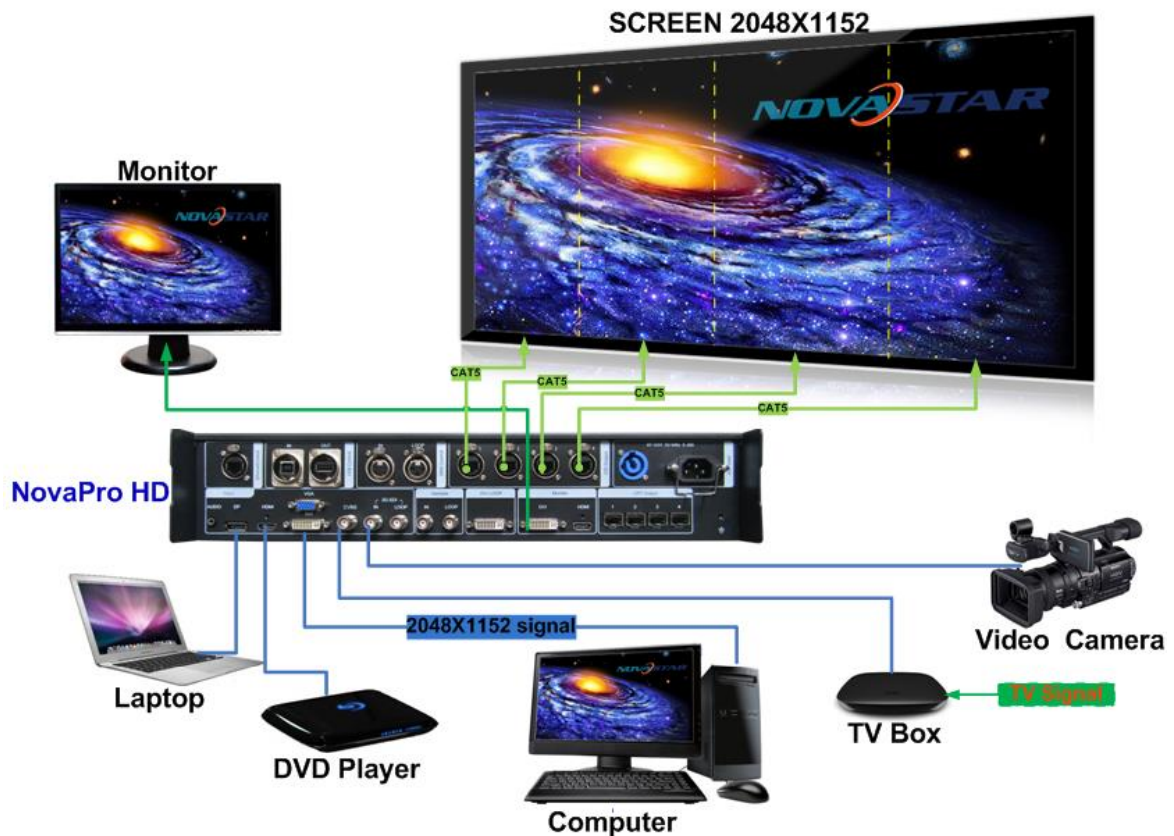
Fig. 4-1 Signal Connection
