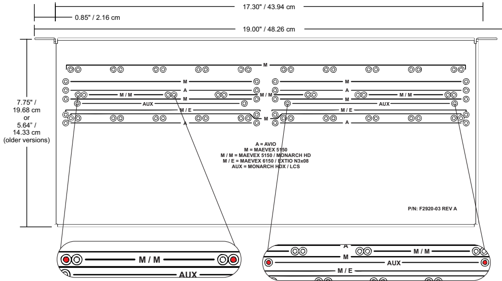
MONARCH HDX and LCS Use the "AUX" holes
