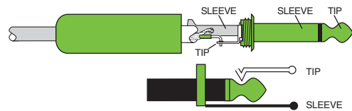
Unbalanced 1/4" TS Connector
