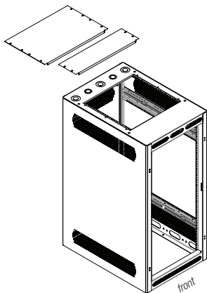
The rack includes a rear door and top closure panels (rear door can be omitted if not needed, see ordering option, pg. 2). A front door is optional, order separately.
