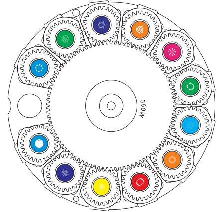
Rotating Gobos (9.9mm outer, 5.5mm inner diameter)
